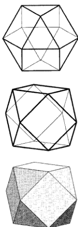
Cuboctaedro
